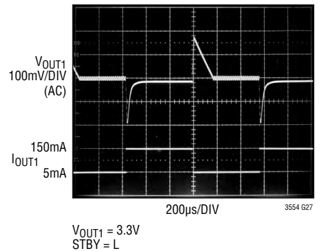
Step-Down Switching Regulator Output Transient
